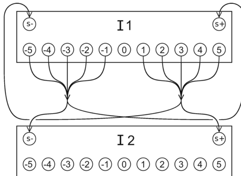
Fig. 15.3 Circuit for the summation of two spatially encoded values. Neurons are drawn as open circles, arrows represent exciting connections. Each box (I1 and I2) represents a Hartmann-Wehner Integrator (see Fig. B 6.1). The left and right shift neurons are displayed as s- and s+, respectively. Two values are initially represented in I1 and I2. After stabilization, the sum of both values is represented in I2. See text for an explanation (after Linder 2005).
