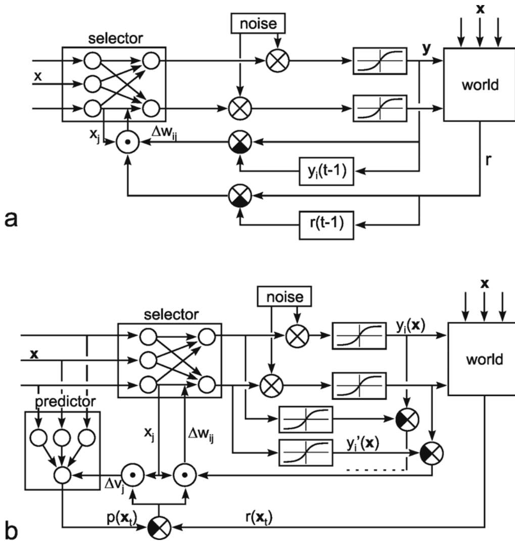
Fig. 12.6 Reinforcement learning. (a) The input vector \mathbf{x} is given to the network, which, in this example, consists of two layers, but might be more complicated. The response of the net is somewhat changed by means of a noise produced by the system. The system contains a memory to store the components of the output vector applied during the previous time step [ y_i(t-1) ]. Furthermore, the system receives a scalar reward signal from the environment (world) and stores the previous reward value r(t-1) . With these values, the appropriate change of the weights w_{ij} can be determined as shown in the lower part of the diagram. (b) If the input vector varies, the application of an additional "predictor net" can solve the problem. In this case, the actual reward is compared with the expected reward p provided by the predictor net. Here, the output vector is not compared with the previous one, but with the original vector that the network proposed before the vector was changed by means of the noise influence. These values can be used to change the weights of the selector net and of the predictor net, accordingly.
