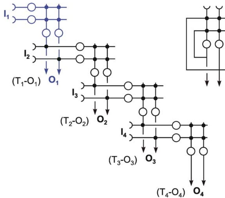
Fig. 12.4 Unfolding a recurrent network in time. To cope with the dynamics of a recurrent network, the net is copied several times, and these copies are connected to form a feedforward net. Each subnet represents another time step. Errors (T_i - O_i) have to be collected for each time step, i.e. for each subnet, and are then used to update the weights
