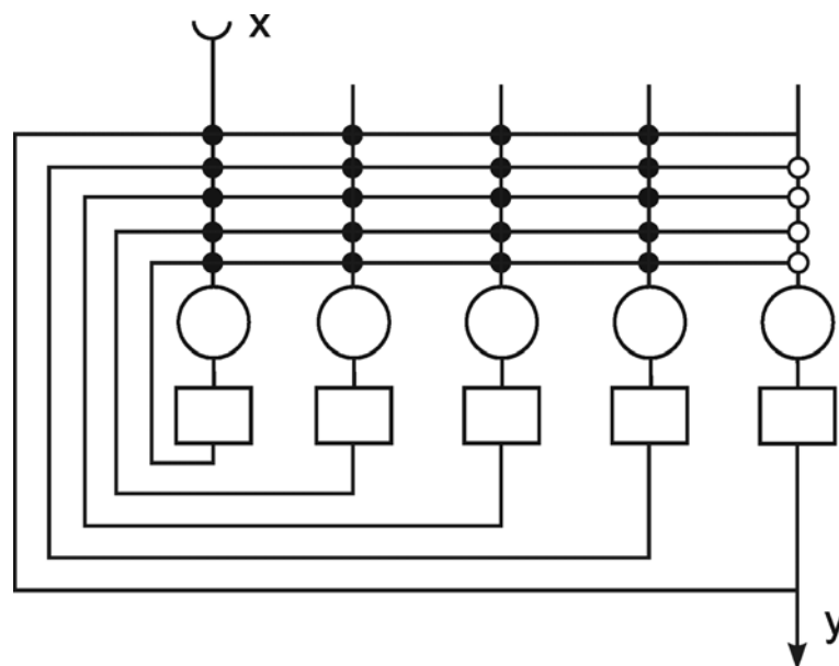
Fig. 14.2 Echo state network. The dynamic reservoir consists of recurrently connected units. The output units are recurrently connected to the units of the dynamic reservoir, but only the output connections (open circles) are due to learning. All the other weights (closed circles) are fixed before learning starts.
