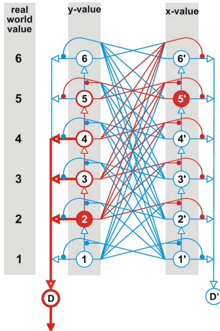
Fig. 15.4 A neural network for the subtraction of two spatially encoded values x - y . Neuroids are drawn as big circles, lines ending in little filled circles represent inhibiting connections. Exciting connections are drawn as arrows. Each unit represents an angular value as indicated on the left. On both sides, the position of the filled neuron represents the y value to be subtracted. Arrows indicate exciting synapses, circles inhibitory synapses. D and D' represent intensity coded output units, each receiving input from every neuroid in its chain. If one neuroid coding for the y value is excited (#2), activation is spread upward to the position opposite to the activated neuroid of the other chain (#5'). Excited elements are shown by red lines. Activation of output unit D is proportional to the absolute value of the difference between x value and y value (and activation of D' for the absolute value of the difference between y value and x value, respectively) (after Linder 2005).
