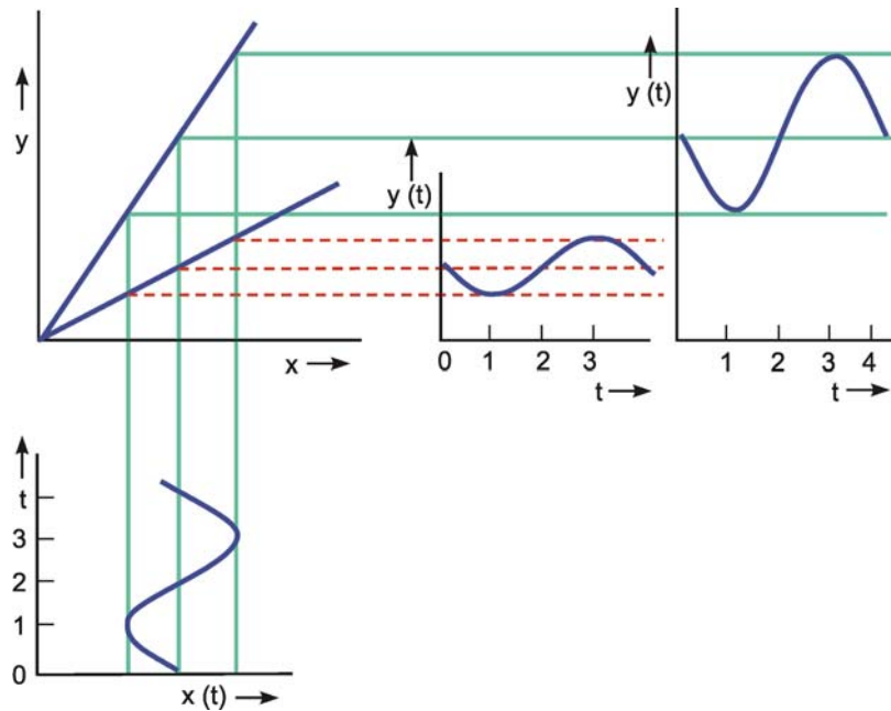
Fig. 5.2 The construction of the output function y(t) for a given input function x(t) , shown for two different linear characteristics
