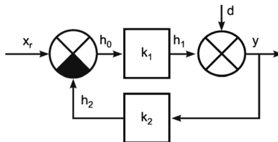
Fig. 8.2 A simplified version of a feedback controller with static elements. x_r reference input, d disturbance input, y control variable, h_0 , h_1 , h_2 auxiliary variables, k_1 , k_2 constant amplification factors
