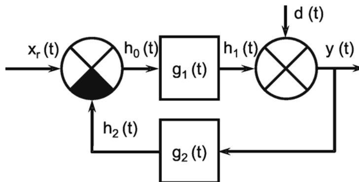
Fig. 8.3 A simplified version of a feedback controller with dynamic elements. x_r(t) reference input, d(t) disturbance input, y(t) control variable, h_0(t) , h_1(t) , h_2(t) auxiliary variables, g_1(t) , g_2(t) weighting functions, describing the dynamic properties of the systems in the feedforward and the feedback channel, respectively
