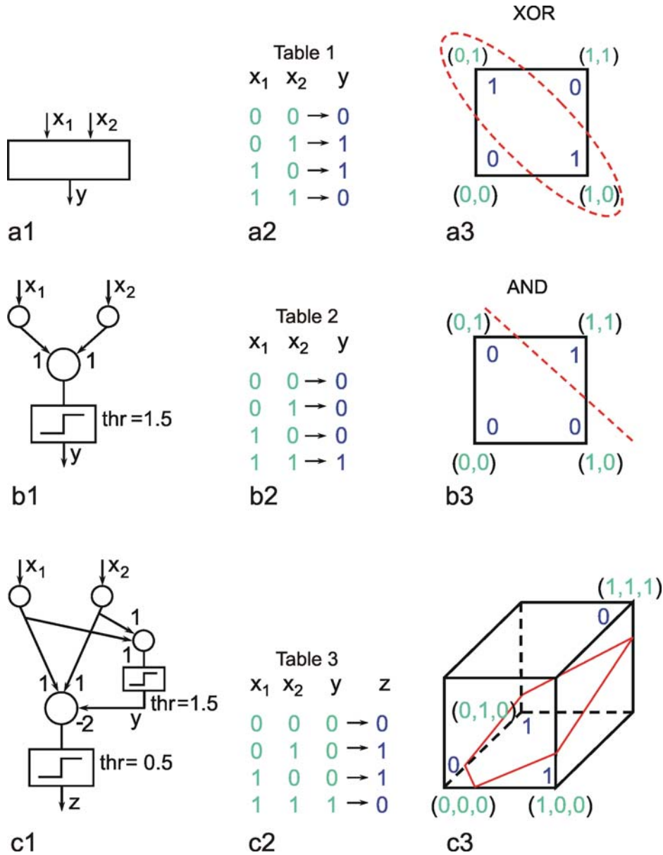
Fig. 10.8 The XOR problem. (a1) A system with two input units and one output unit should solve the four tasks presented in the Table (a2). These tasks are illustrated in geometrical form (a3) such that the four input vectors are plotted in a plane and the required output values are attached to their input vectors. The two input vectors which should produce an output value of one are circled. (b1) A two-layer system solving the AND problem. As in (a), the tasks to be solved are shown in Table (b2) and in geometric form in (b3). The network (b1) can solve the AND problem using the weights shown and a Heaviside activation function with a threshold of 1.5. (c) A three-layer system can solve the XOR problem, when, for example, the weights and threshold values shown in (c1) are applied. The output y of the hidden unit corresponds to that of the AND network (b1) (see Table c2). The input vector of the final neuroid, representing the third layer, is three-dimensional. Therefore, geometrically the input-output situation of this unit has to be illustrated using a three-dimensional representation. As above, the four input vectors are marked together with the expected output. The oblique plane separates the two vectors producing a zero output from the two others which produce unity output. Such a linear separation is not possible in (a3)
