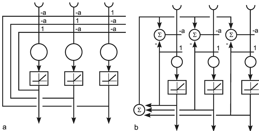
Fig. 11.3 A recurrent winner-take-all network consisting of three units (a). A formally identical system with four extra units (b). Rectifiers (Fig. 5.8) are used as activation functions
