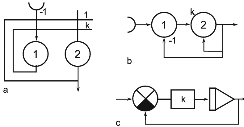
Fig. 11.7 An asymmetrical recurrent network with the properties of a temporal low-pass filter (a). (b) and (c) show the same system but are redrawn to allow comparison with figures of Chapter 8. For easier identification the two units are numbered in (a) and (b)
