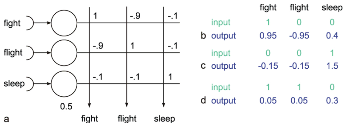
Fig. 16.2 A winner-take-all net with unequal inhibitory influences. (a) The net has to decide which of three behavior agents (inputs fight, flight, and sleep) finally controls the activity, i. e., the output. The sleep agent is assumed to obtain a constant bias of 0.5. If only the fight agent (b), the flight agent (not shown) or only the sleep agent (c) is activated, the output corresponds to the input situation. (d) If fight and flight are equally active, the sleep agent will win. This simulates the occurrence of displacement behavior
