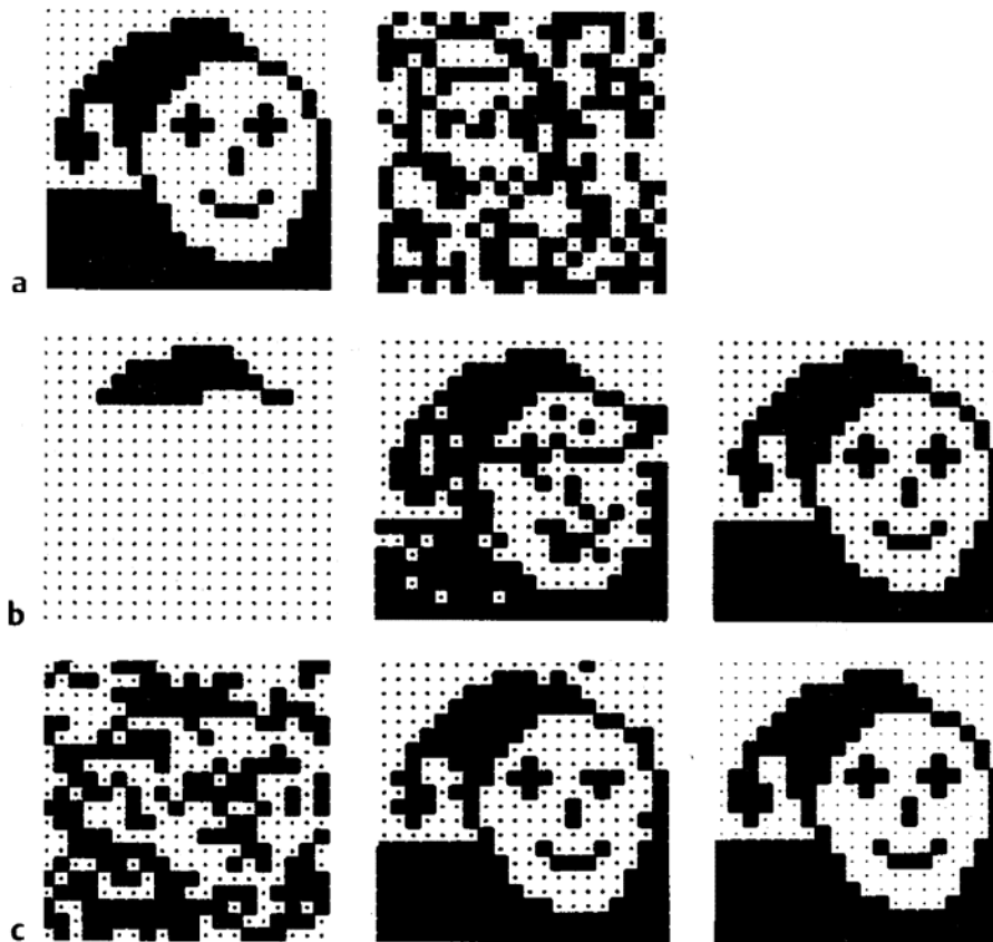
Fig. 11.5 Pattern completion. (a) The Hopfield net consists of 20 \times 20 neuroids, which can show two states, illustrated by a dot or a black square, respectively. The weights are chosen to store 20 different patterns; one is represented by the face, the other 19 by different random dot patterns. (b) After providing only a part of the face pattern as input (left), in the next iteration cycle the essential elements of the final pattern can already be recognized (center), and the pattern is completed two cycles later (right). (c) In this example, the complete pattern was used as input, but was disturbed by noise beforehand (left). Again, after one iteration cycle the errors are nearly corrected (center), and the pattern is complete after the second iteration (right) (Ritter et al. 1992)
