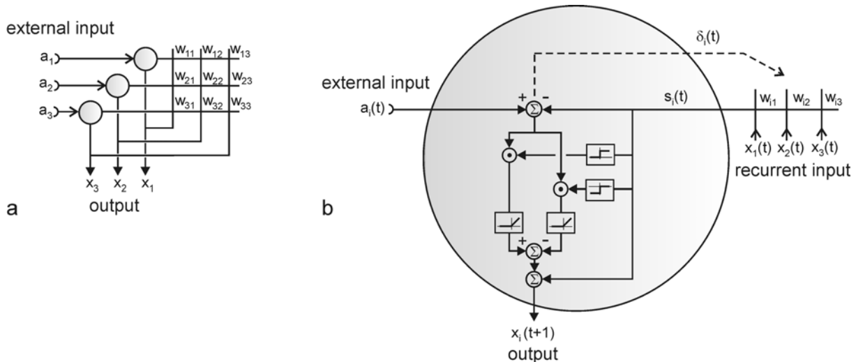
Fig. 12.5 Recurrent network with IC units. (a) A network containing 3 units. (b) The circuit characterizing an IC unit
