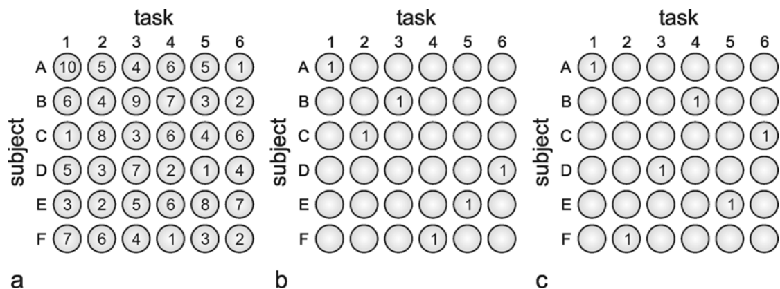
Fig. 11.4 Six subjects A - F have to perform six tasks 1-6. To solve the optimization problem, 6 x 6 units are arranged in six lines, one for each subject (a). The vertical columns correspond to the tasks to be performed. The number in each unit shows a measure for the qualification of each subject and each task. These numbers represent the input values. The units are connected such that the six units of a line as well as the six units of a column form winner-take-all nets. Furthermore, an additional unit computes the sum of the activations of all these 36 units (as shown in Fig. 11.3b) including an offset value. This sum is fed back to all 36 units. (b) An almost optimal solution found by this network. The sum of the qualification measures is 40 in this case. The optimal solution is shown in (c) with a total qualification of 44 (Tank and Hopfield 1987)
