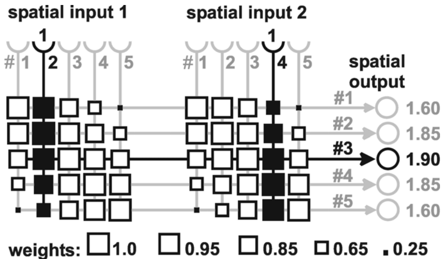
Fig. 15. 2 Calculating the mean value of two spatially encoded scalar. Output neuroids are drawn as open circles, input neuroids as semicircles. Arrows represent exciting connections, the weights are represented as squares. Two spatially encoded scalars "2" and "4" are given by an excitation of 1.0 of the respective neuroids (black pathways, input neuroid #2 and #4, respectively). In that case, the highest activation can be found in output neuroid #3. If necessary, the mean value can be computed by a winner-take-all network (not shown) at the right side (after Linder 2005 ).
