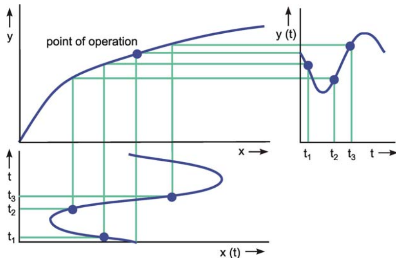
Fig. 5.3 The construction of the output function y(t) for a given input function x(t) , shown for a nonlinear (in this case logarithmic) characteristic. As example, three time values t_1 , t_2 and t_3 are marked. The point of operation is defined as the mean of the input function (after Varju 1977)
