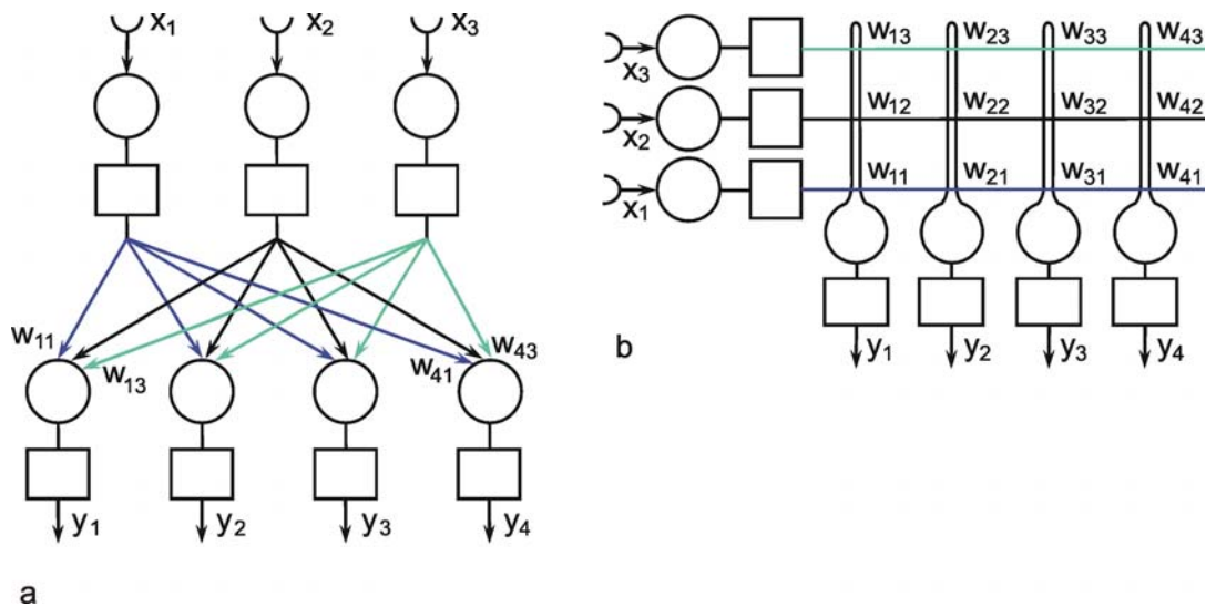
Fig. 9.2 A two-layer feedforward network with n (= 3) units in the input layer and m (= 4) output units in the output layer. x_i represent the input values, y_i the output values. The weights w_{ij} have two indices, the first corresponds to the output unit, the second to the input unit. As in Fig. 9.1, (a) more resembles the arrangement of a net of biological neurons, whereas the matrix arrangement of (b) permits a clearer illustration of the connections and the weights (only some weights are shown in (a)). The boxes represent unspecified activation functions
