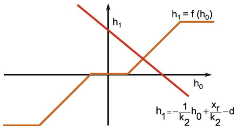
Fig. 8.4 Graphical solution of input-output relation of a negative feedback system with a nonlinear characteristic f(h_0) in the feedforward channel. Equation (7) is graphically illustrated by the red line. Its position depends on the values of the parameters x_r and d . Changing these parameters results in a parallel shift of this line. As an example, the nonlinear characteristic h_1 = f(h_0) is endowed with threshold and saturation (yellow lines). For given values x_r and d the intersection of both lines indicates the resulting variable h_1 . Equation(4) ( y = h_1 + d ) allows determination of the value of the actual output
