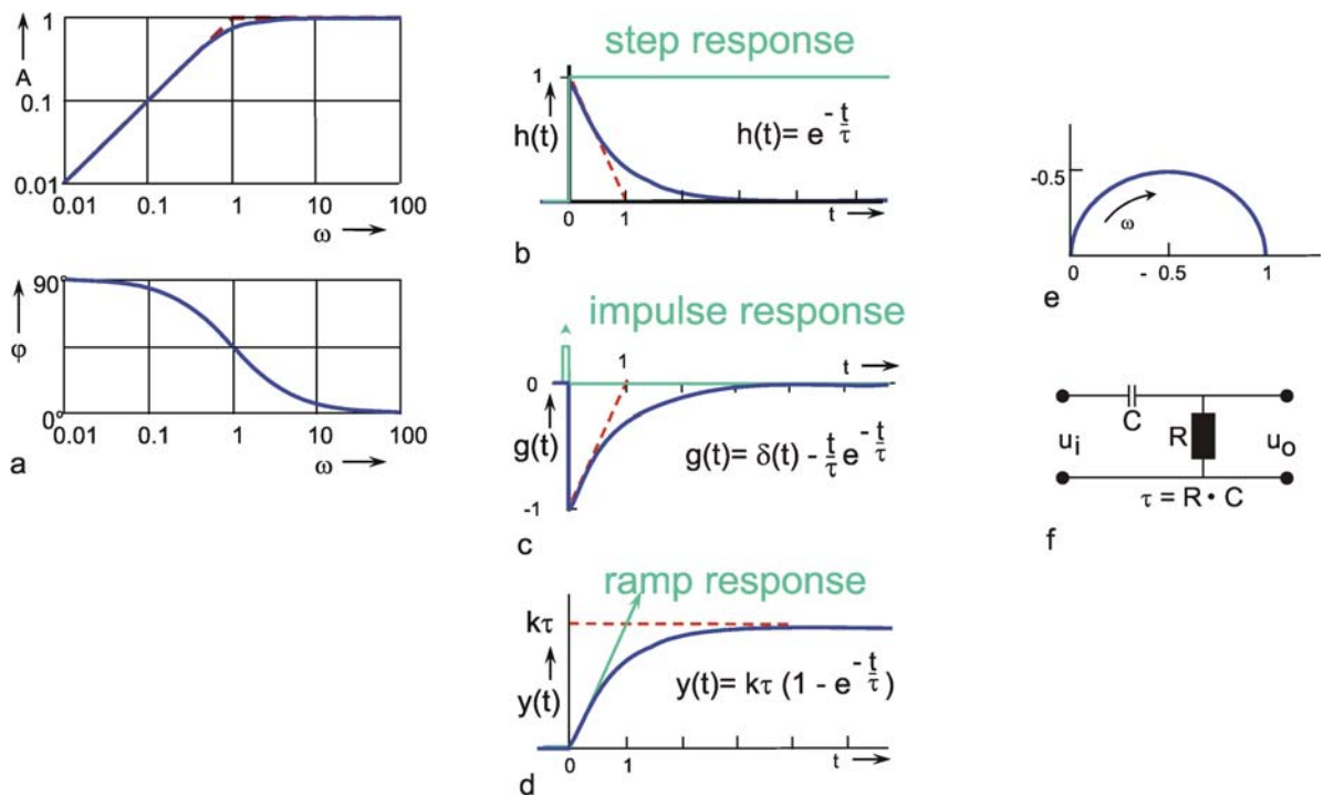
Fig. 4.3 High-pass filter. (a) Bode plot consisting of the amplitude frequency plot (above) and the phase frequency plot (below). Asymptotes are shown by red dashed. A amplitude, \phi phase, \omega = 2\pi\nu angular frequency. (b) step response, (c) impulse response, (d) ramp response. In (b) - (d) the input functions are shown by green lines. The formulas given hold for t > 0 . k describes the slope of the ramp function x(t) = kt . (e) polar plot. (f) Electronic wiring diagram, R resistor, C capacitor, \tau time constant, u_i input voltage, u_o output voltage
