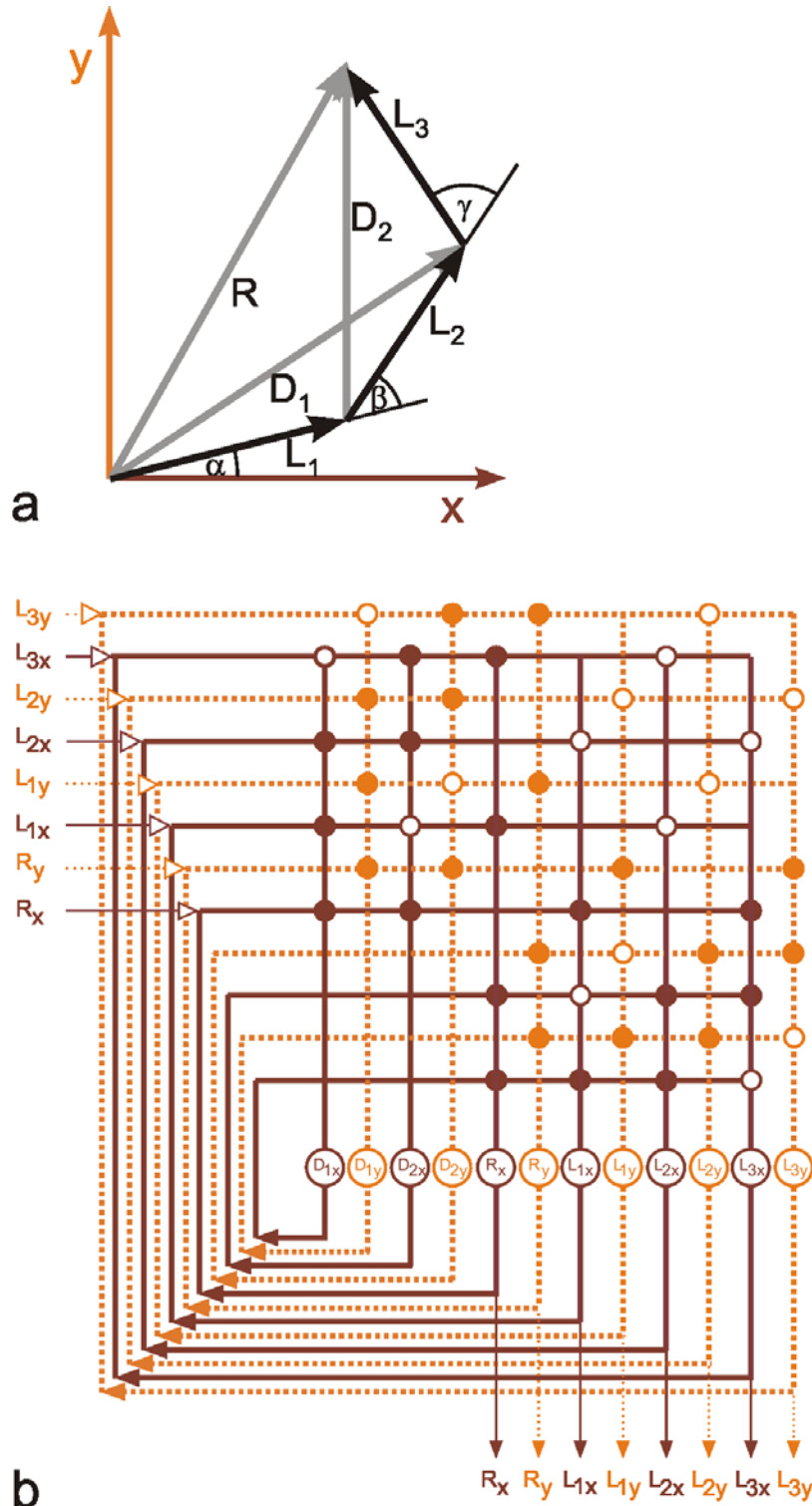
Fig. 14.4 (a) An arm consisting of three segments described by the vectors L_1 , L_2 , and L_3 which are connected by three planar joints. The joint angles are \alpha , \beta , and \gamma . The position of the endeffector is described by R . Furthermore, two additional vectors D_1 and D_2 , describing the diagonals, are shown. (b) The linear version of the MMC net. The output values represent the components of the vectors R , L_1 , L_2 , and L_3 (lower line). Solid lines represent the subnet for the x components, dashed lines that for the y components. To calculate the inverse kinematics, the components of R have to be provided as input for the net. However, any other combination of input values could be chosen instead. The possible input values are shown on the vertical column at the left. For the chosen input, the recurrent line is suppressed, and only the input value is fed into the net, symbolized by the small arrowheads.
