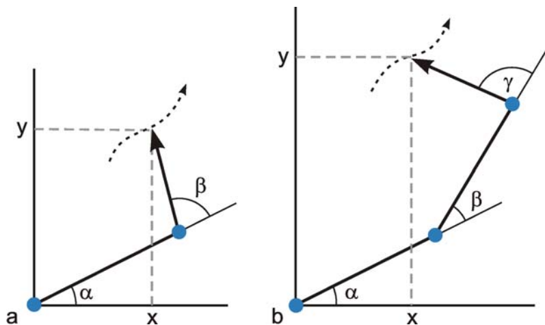
Fig. 14.6 A two-joint arm (a) and a three-joint arm (b) moving in a two dimensional ( x - y ) plane. When the tip of the arm has to follow a given trajectory (dotted arrow), in the redundant case (b) an infinite number of joint angle combinations can solve the problem for any given position of the tip.
