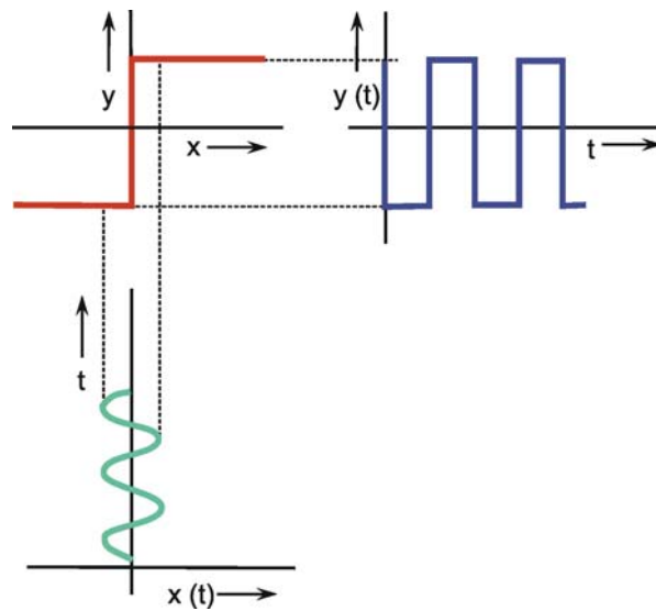
Fig. 5.12 An all-or-none characteristic corresponding to the Heaviside function. x(t) input function, y(t) output function
