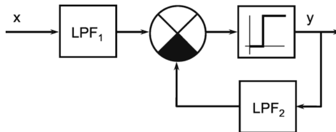
Fig. 8.17 A simple system for the simulation of a spiking neuron. LPF 1 , and LPF 2 represent two low-pass filters. As soon as the threshold of the Heaviside function is overcome, a spike is elicited
