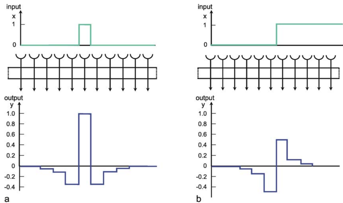
Fig. 10.4 Impulse response (a) and step response (b) of a two-layer feedforward network as shown in Fig. 10.3, but with lateral connections including three neighbors instead of only one (spatial high-pass filter). The network is shown as a box. The central weight is 1. The weight values decrease symmetrically to right and left, showing values of -0.35, -0.1, and -0.05, respectively. These values can be directly read off the output, when a "spatial impulse" (a) is given as input, i. e., only one unit is stimulated by a unity excitation. Input ( x ) and output ( y ) functions are shown graphically above and below the net, respectively
