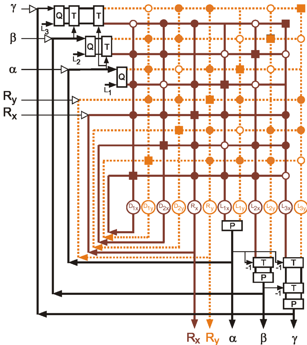
Fig. 14.5 The MMC net as shown in Fig. 14.4b, but with nonlinear subsystems in the feedback loops. In this case the input and output vectors contain the components R_x and R_y , describing the position of the endeffector, as well as the joint angles \alpha , \beta , and \gamma . The nonlinear systems P, T, and Q are explained in the text.
