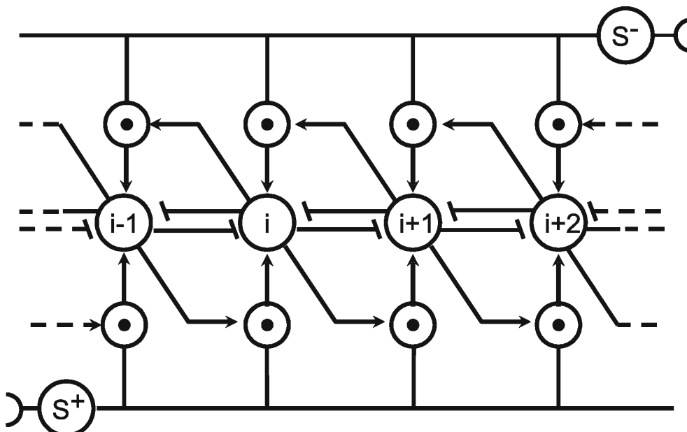
Fig. B 6.1 A simple network for spatial integration. The input unit s^+ monitors the movement in one direction, the unit s^- that in the opposite direction. By excitation of s^+ , the position of the excited neuroid of the chain is moved to the right, whereas it is shifted to the left, if s^- is excited. Therefore, the position of the excited neuroid represents the integral of the input signal s
