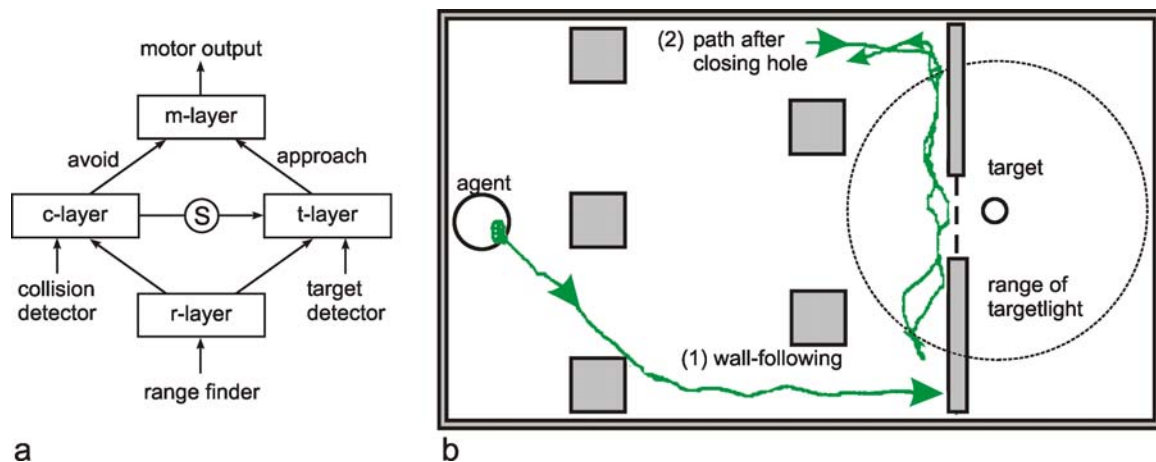
Fig. 16.6 (a) The structure of a robot to learn a new reflex. Two reflexes are built into the system: a connection between the collision detector and the motor output, producing an avoidance reflex, and a connection between target detector and motor output, producing a reaction to approach the target. In the case of a conflict the former reflex suppresses the latter (S). The connection between a third group of sensors, the range finder, and the other reflexes are learnt "automatically" using Hebbian learning. (b) shows some examples of how the robot behaves. It shows wall following (trace 1). Usually the robot finds the target after it has reached the range of target light source. If, in another experiment (trace 2), the hole in front of the target is closed, the robot "searches" in front of the closed door. As the collision avoidance net is stimulated quite often, the suppression of the approach net may become inhibited and the robot may move outside the range of the target light source (after Pfeifer and Verschure 1992, Pfeifer 1995)
