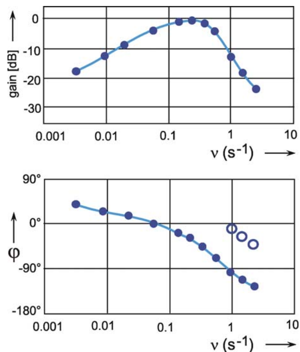
Fig. B 1.1 Bode plot of the forces developed by the neck muscles of a locust. Input is the position of a sinusoidally moved visual pattern. \nu is stimulus frequency. The gain is measured in dB (after Thorson 1966)
