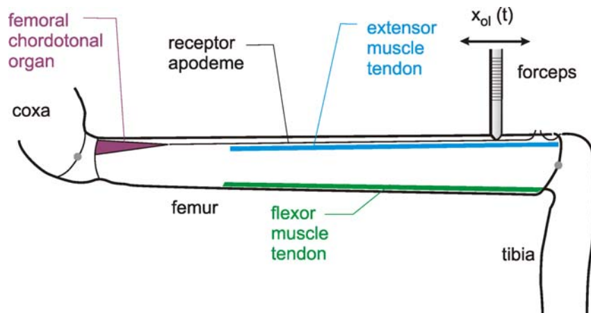
Fig. 8.6 Morphological basis of a resistance reflex in the leg of an insect. The angle between femur and tibia is monitored by the femoral chordotonal organ, which is mechanically connected to the tibia by a long receptor apodeme. By cutting this apodeme, the loop can be opened and the apodeme can be moved experimentally using a forceps and thus the x_{ol} input can be applied (Bässler 1983)
