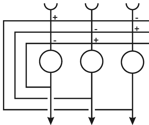
Fig. 11.6 An asymmetrical recurrent network showing rhythmic behavior. After the excitation of one unit, the three units are excited in cyclic order
