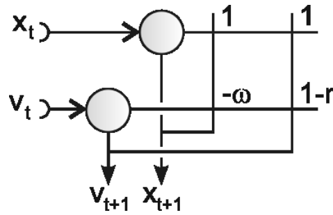
Fig. 14.3 A recurrent net showing damped oscillations. \omega frequency, r friction
