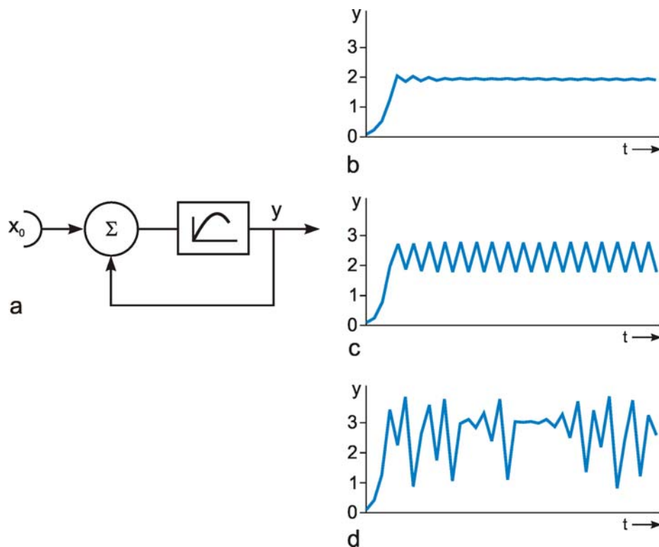
Fig. 11.10 A recurrent system can show chaotic behavior. (a) The system containing a nonlinear characteristic of the form y = a_1x - a_2x^2 . (b - d) Temporal behavior of the system for different parameters of the nonlinear characteristic. (b) a_1 = 2.5 , (c) a_1 = 3.2 , (d) a_1 = 3.8 . a_2 is 0.2 and the starting value x_0 = 0.1 for all cases
