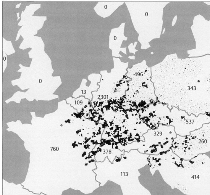
Fig. B 5.2 Spotty distribution of rabies (dots) in central Europe in the year 1983. In brackets: number of counts. The data from Poland and the former DDR are not comparable with the others because they were collected over larger spatial units (after Fenner et al. 1993 ; courtesy of the Center for Surveillance of Rabies, Tübingen, Germany)
