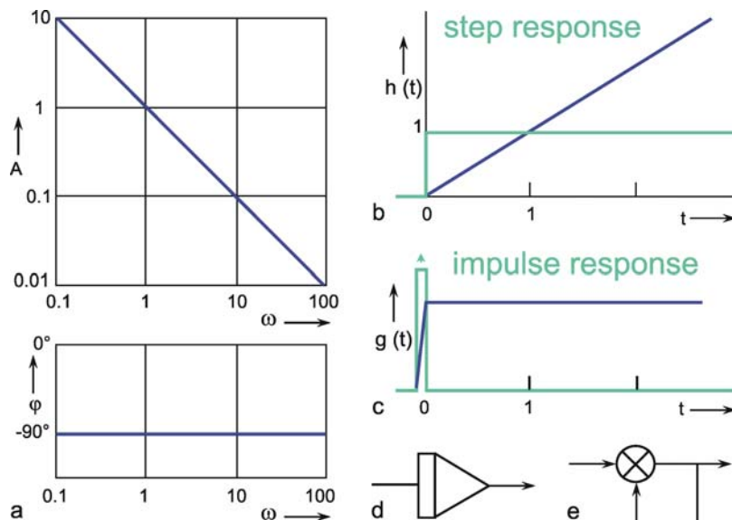
Fig. 4.13 Integrator. (a) Bode plot, A amplitude, \phi phase, \omega angular frequency. (b) step response. (c) Impulse response. In (b) and (c) the input functions are shown by green lines. (d) symbolic representation of an integrator. (e) An integrator can also be realized by a recurrent summation
