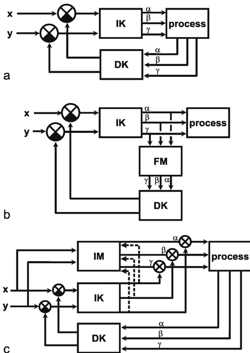
Fig. 14.7 Three ways of controlling the movement of a redundant (or non redundant) arm as shown in Fig. 14.6. DK, IK: networks solving the direct or inverse kinematics, respectively. FM: forward model of the process. IM: inverse model of the process. The dashed lines in (c) denote the error signals used to train the inverse model
