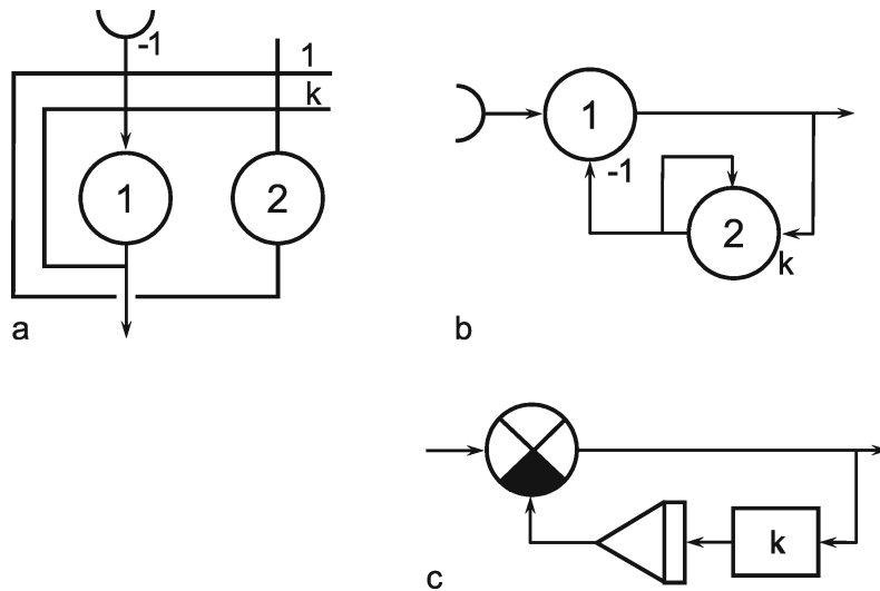
Fig. 11.8 An asymmetrical recurrent network with the properties of a temporal high-pass filter (a). (b) and (c) show the same system but are redrawn to allow comparison with figures of Chapter 8. For easier identification the two units are numbered in (a) and (b)
