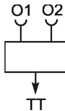
Fig. B 2.1 The elementary movement detector. Two ommatidia, O1 and O2, form the input; the turning tendency TT represents the output of the system
