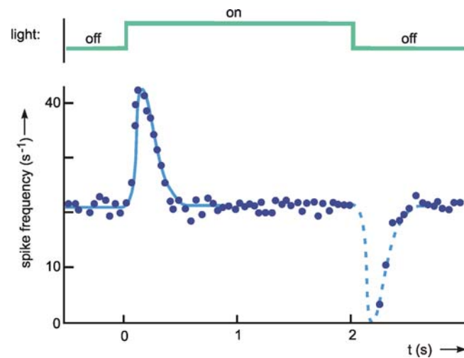
Fig. 4.4 The response of a single fiber of the optical nerve of Limulus . As input function light is switched on for 2 seconds (upper trace). The output function shows the instantaneous spike frequency (each dot is calculated as 1/\Delta t , \Delta t being the time difference between two consecutive spikes). The solid blue line shows an approximation of the data. The dashed part (response to the decreasing step) represents the mirror image of the first part of the approximation (after Ratliff 1965). Note that negative spike frequencies are not possible
