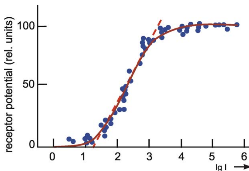
Fig. 5.4 The dependency of the receptor potential of a retinal sensory cell of a turtle (ordinate) on the intensity of the light stimulus (abscissa, logarithmic scale). The central part can be approximated by a straight line (dashed), indicating the logarithmic part of the characteristic (after Schmidt 1973)
