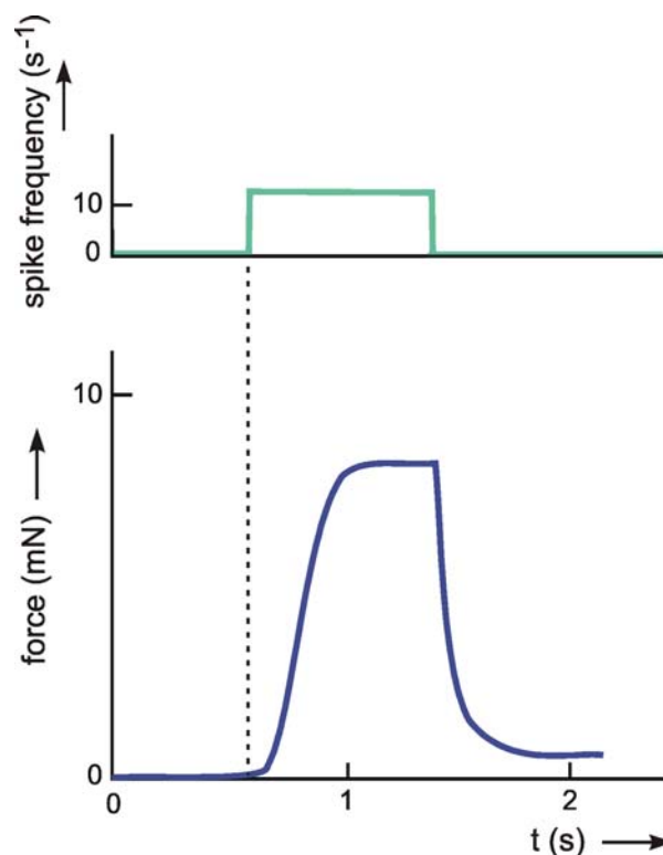
Fig. 4.2 The response of an insect muscle to an increasing and a decreasing step function. The input function (upper trace) is given by the experimentally induced spike frequency of the motoneuron. The output function (lower trace) shows the force developed by the muscle (after Iles and Pearson 1971 )
