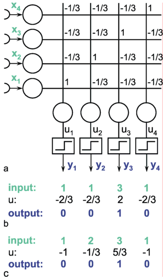
Fig. 10.6 A feedforward winner-take-all network (a) . The weights at the diagonal are 1. Because the net consists of four neuroids in each layer, all other weights have a value of -1/3 . (b) and (c) show two examples of input values (upper line), the corresponding summed excitations u_i (middle line) and the output values after having passed the Heaviside activation function (lower line). In the example of (b) the threshold of the activation function could be any value between -2/3 and 2. For (c) this threshold value has to lie between 1/3 and 5/3
